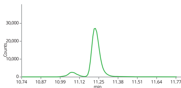
Lycopsamine N-oxide (316.2->111.0)
