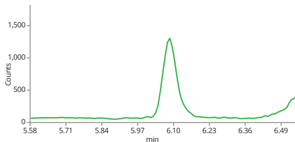
Intermedine N-oxide (316.2->172.0)
