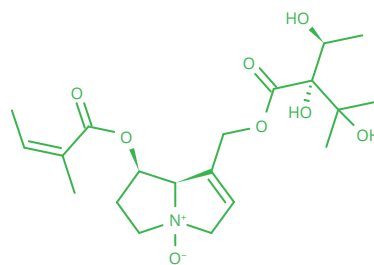
Echimidine N-oxide
