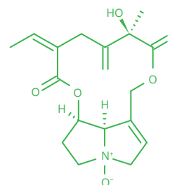
Seneciophylline N-oxide
