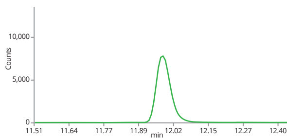
Lycopsamine N-oxide (316.2->111.0)
