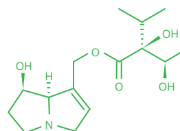
Intermedine
