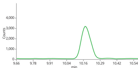
Lycopsamine N-oxide (316.2->111.0)
