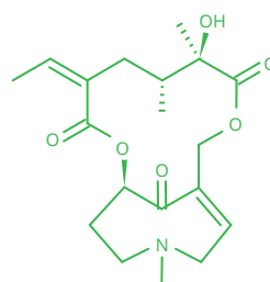
Senkirkine
