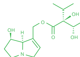
Lycopsamine
