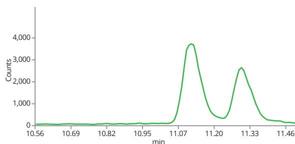
Intermedine N-oxide (316.2->111.0)
