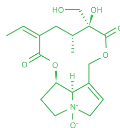
Retrorsine N-oxide
