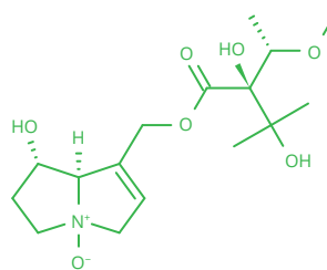
Europine N-oxide
