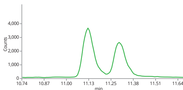
Intermedine N-oxide (316.2->111.0)
