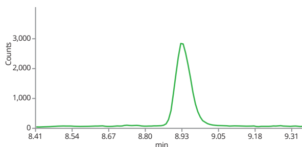
Intermedine N-oxide (316.2->94.0)
