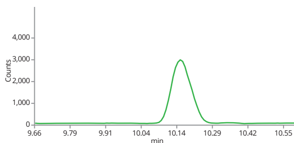
Lycopsamine N-oxide (316.2->94.0)
