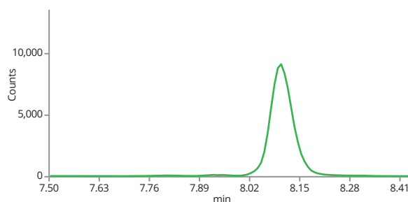
Lycopsamine N-oxide (316.2->111.0)
