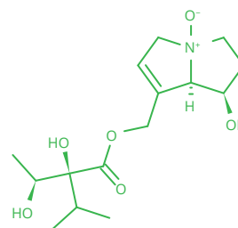
Lycopsamine N-oxide
