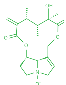
Senecivernine N-oxide
