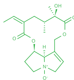
Senecionine N-oxide
