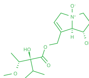
Heliotrine N-oxide
