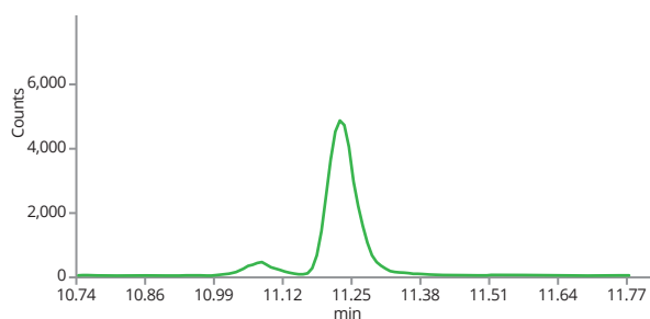
Lycopsamine N-oxide (316.2->172.0)
