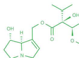
Heliotrine
