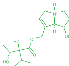
Intermedine N-oxide
