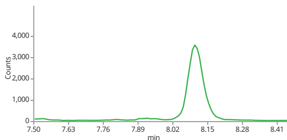
Lycopsamine N-oxide (316.2->172.0)
