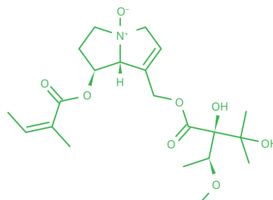
Lasiocarpine N-oxide
