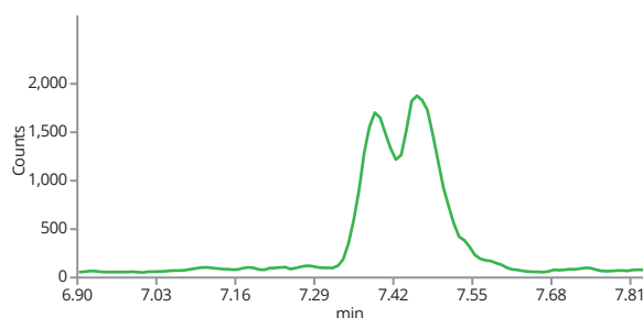
Intermedine N-oxide (316.2->111.0)
