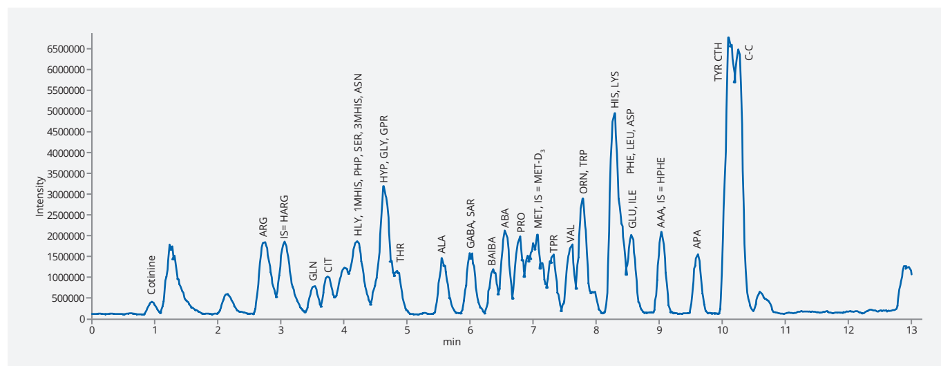
Fig. 1: Standard mixture – LC MetAmino ® kit; mass extracted chromatogram; 5 nmol SD1 and SD2 according to the manual [2]
