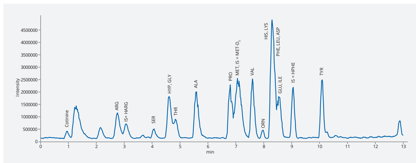
Fig. 2: Fish feed hydrolysate – LC MetAmino ® kit; mass extracted chromatogram; (30 µg of sample after recalculation)
